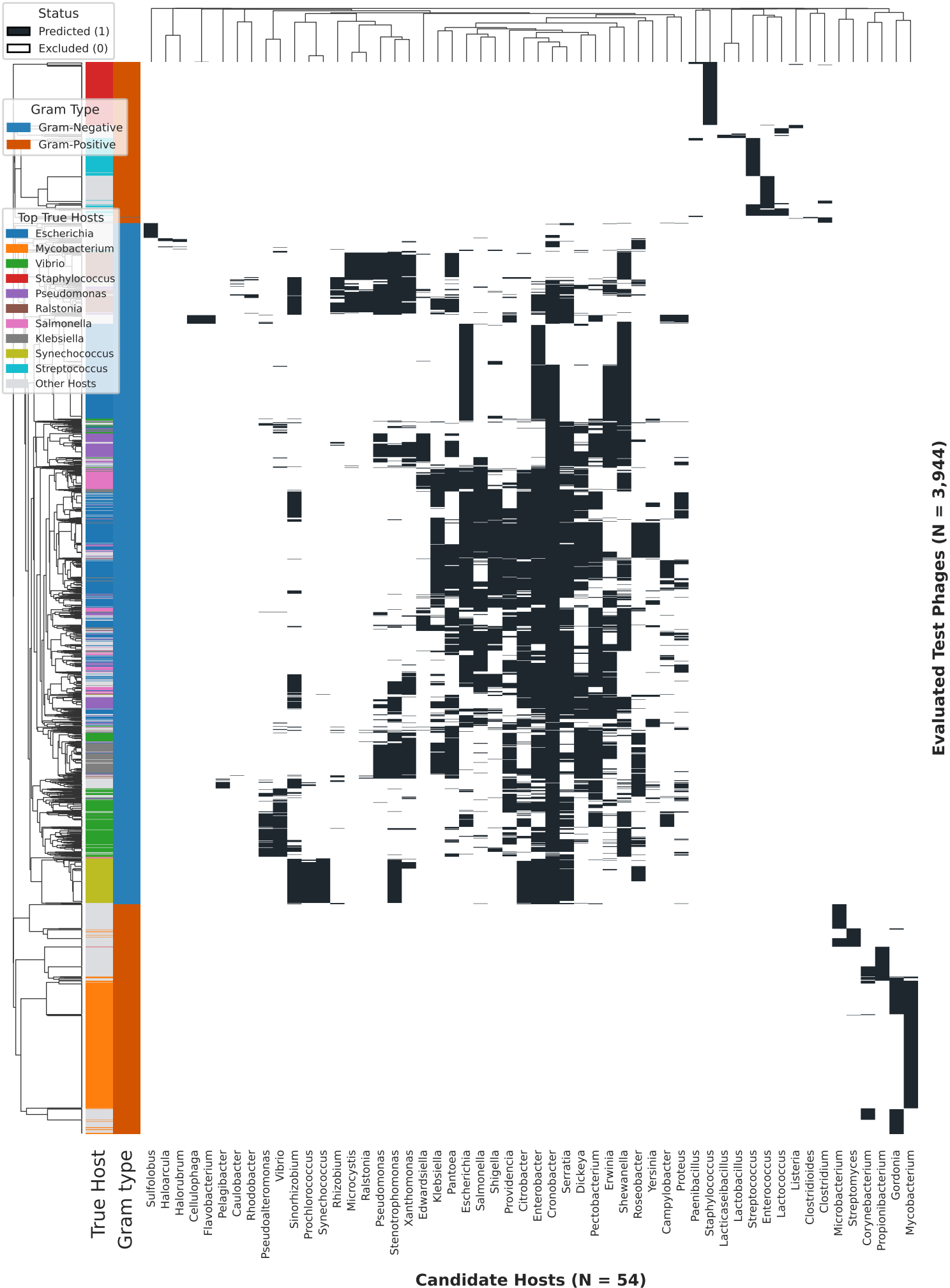
Clustermap of Predicted Phage Host Interactions (Collapsed 1D)
